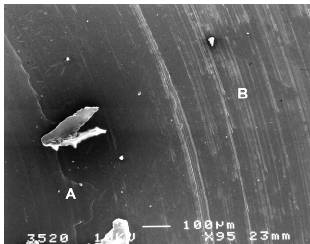
Fig. 14. A closeup of the beginning of the outer wear tracks with the edge of a transfer film and fibril formation evident.
