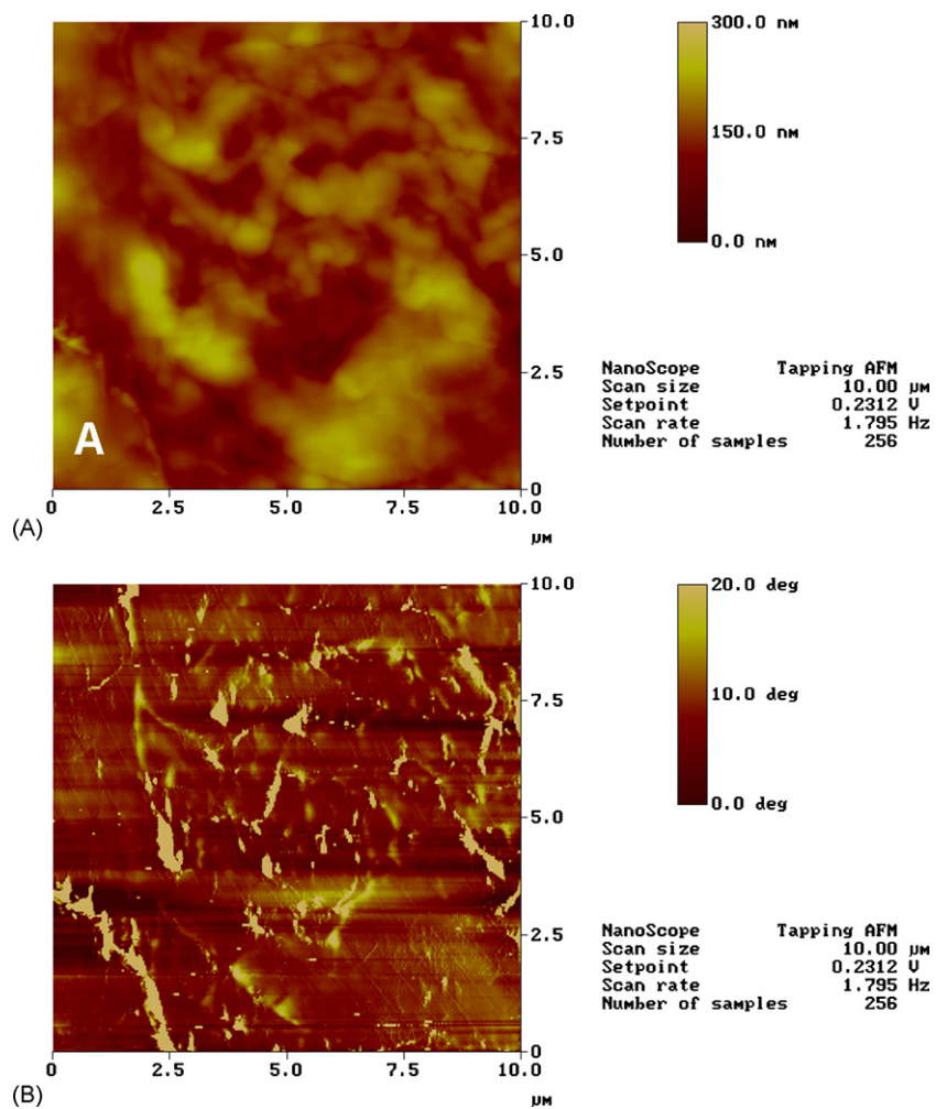
Fig. 17. (A) The top of the polymer wear slope with large plastic features and some delamination. (B) Phase view showing a high response from the delamination.
