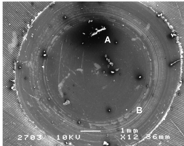
Fig. 12. Wide view of the polymer disc wear area with flakelet debris and adhesive wear fibrils on the outer wear slope.
