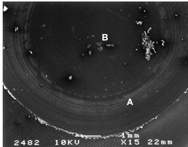
Fig. 13. A closeup on the outer region of the polymer disc wear area showing fatigue flakelets, adhesive wear fibrils and debris buildup on the edge of the wear area.
